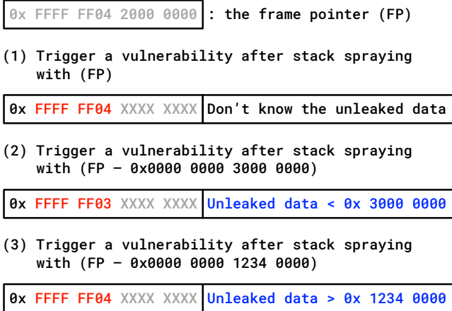
Figure 3: The procedure for identifying a kernel stack address using the kernel stack spraying via a BPF program. By checking changes of the leaked data, we figure out possible ranges of the leaked data until the stack base address is revealed.
